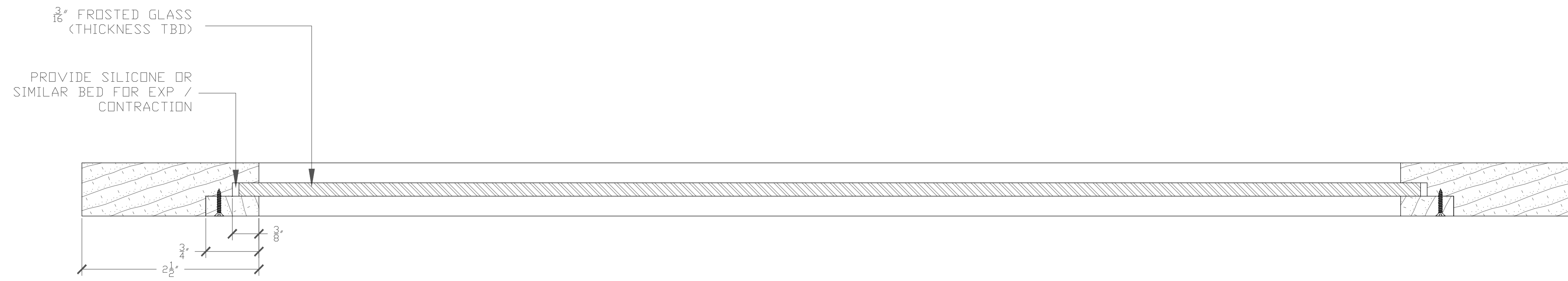
1 WINDOW GLASS SECTION Scale: FULL SIZE
